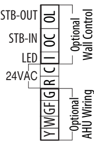
Wiring diagram
