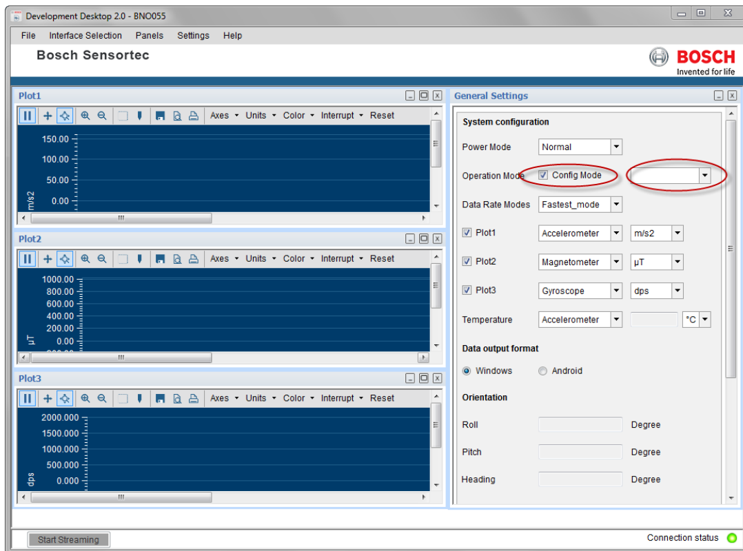
Figure 3 : Main window of Development Desktop
