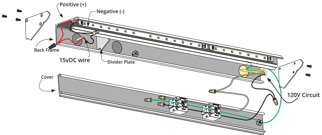
18-1/2" Fixture Shown
