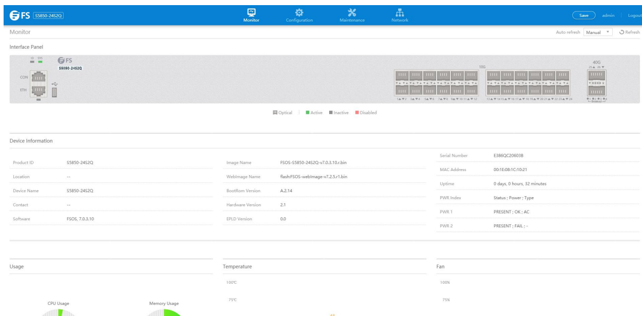
Figure 3 Monitor page
