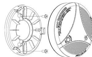
Figure 9: Mounting the bracket
