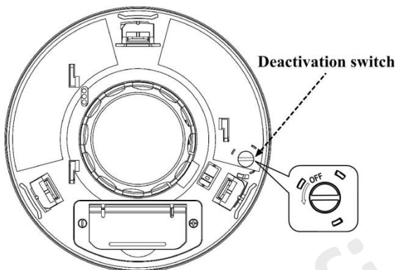
Figure12: Location of deactivation switch for model
