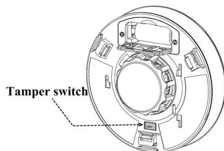
Figure11: Tamper switch location
