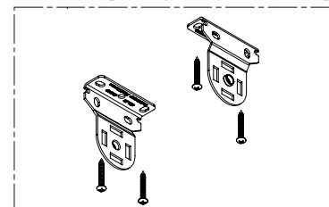
Figure 3. Install Brackets
