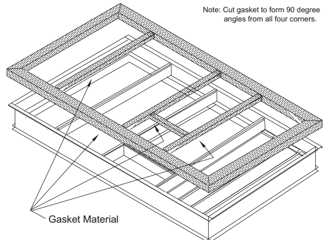
Figure 7. Installing gasket material
