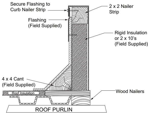
Figure 4. Typical installation on existing construction
