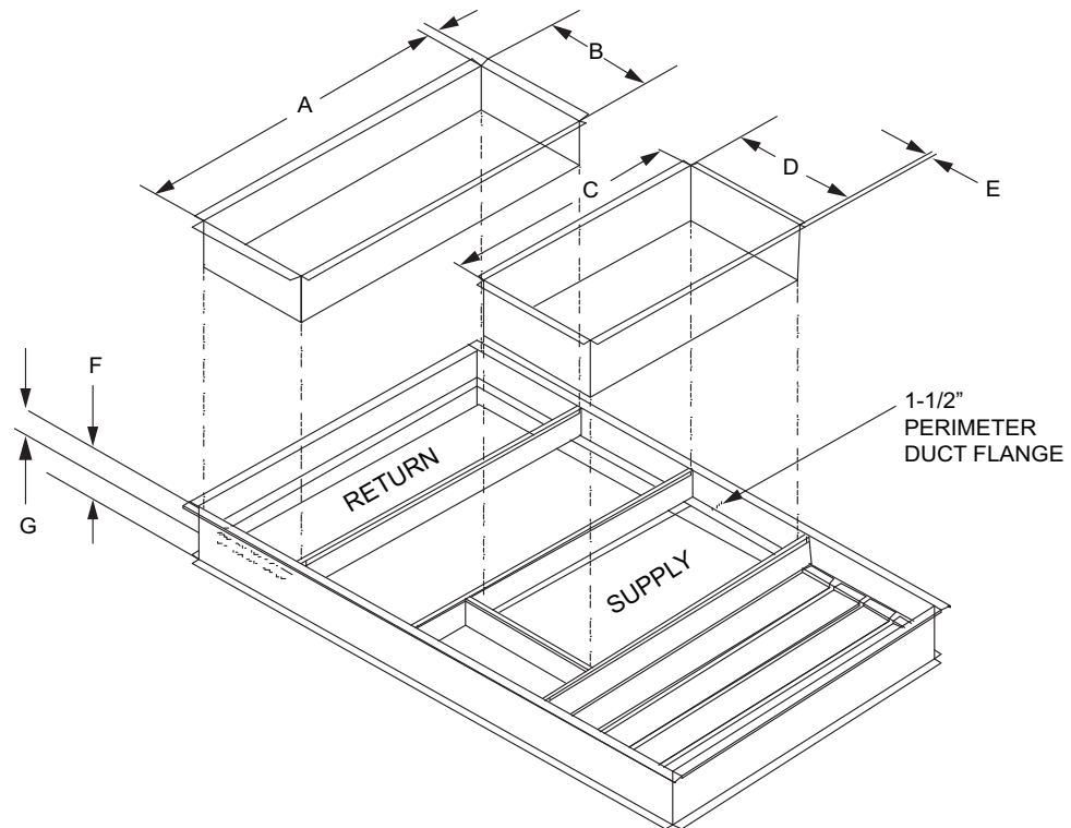
Figure 8. Duct dimensions
