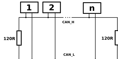
Fig. 26: Termination diagram.
