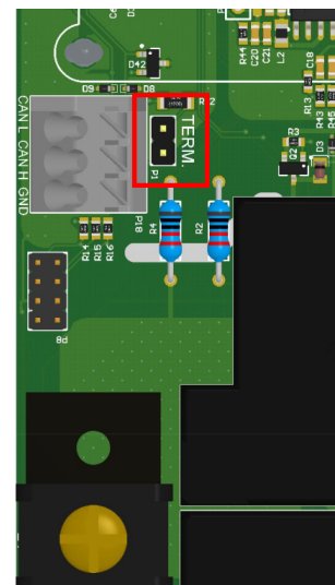
Fig. 28: The place of applying the terminating jumper (variant A)
