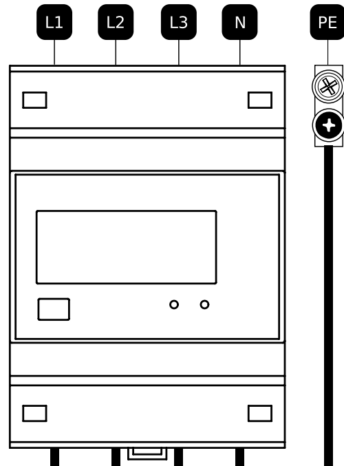
Fig. 18: Recommended connection when applying a MID meter.
