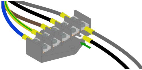
Fig. 15: Connection using fork terminals
