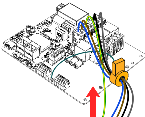
Fig. 21: RCM B connection
