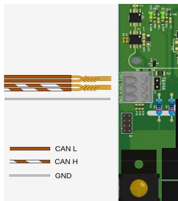
Fig. 24: Diagram of Enelion Chain communication cables connection (variant A)
