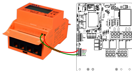
Fig. 19: MID meter communication connection.
