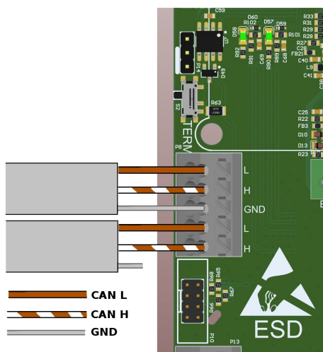
Fig. 25: Diagram of Enelion Chain communication cables connection (variant B)
