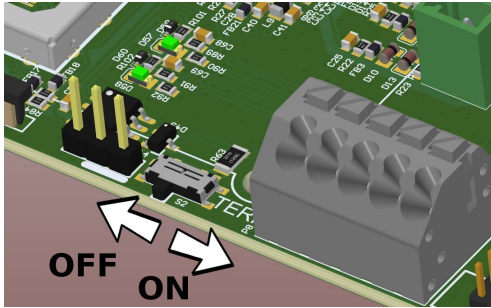
Fig. 29: The place of applying the terminating jumper (variant B)
