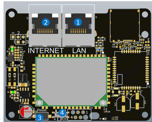
Fig. 31: Enelion Bridge module diagram.
