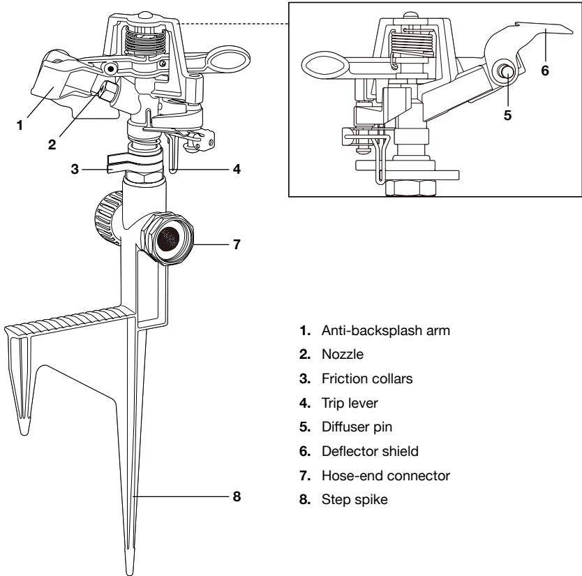
Sprinkler Head
