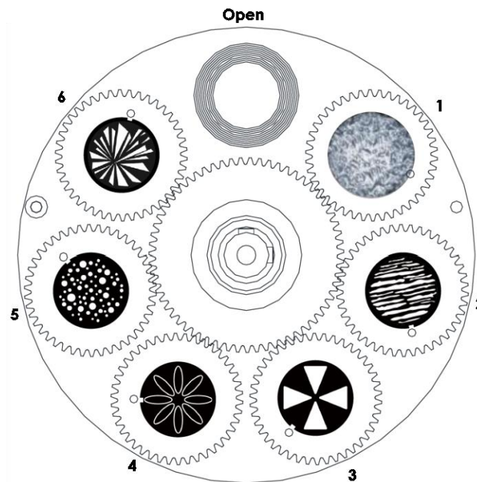
Figure 8. Gobo Wheel 2
