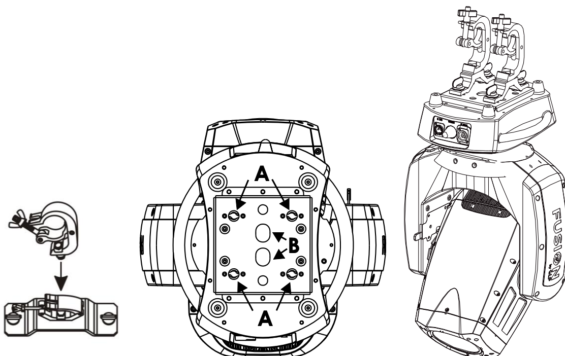
Figure 4. Omega bracket fasteners
