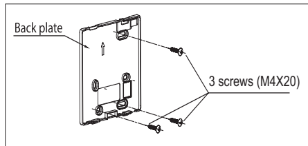
Figure 3. Securing Back Plate to Drywall
