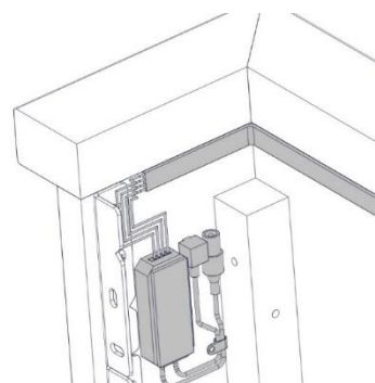
Power Cable
