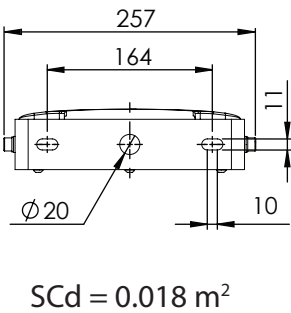
Floodlight console
