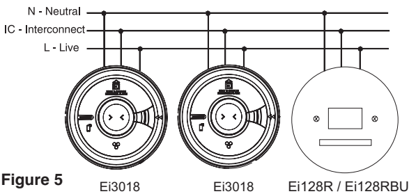
Figure 5 The above shows the connection for Carbon Monoxide Alarms. Connect the Smoke/Heat Alarm similarly but on a separate circuit to the Carbon Monoxide Alarm (unless an Ei1529RC Control Switch is used on the system)
