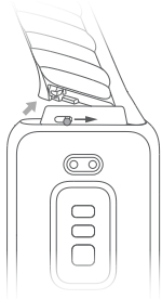
Remove strap
