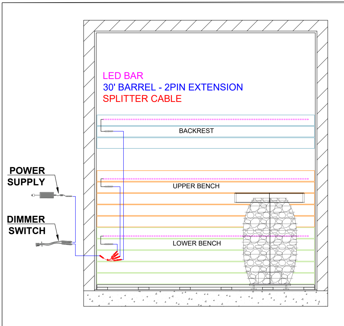
Figure 5: Connections Diagram 2
