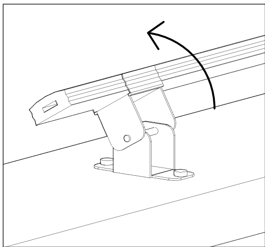
Figure 10: LED Tilting
