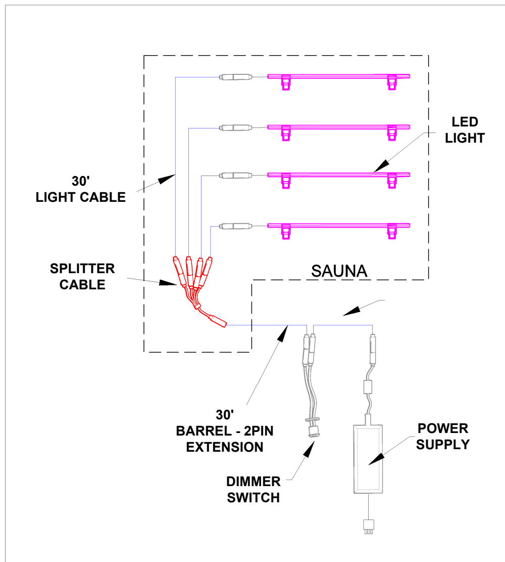
Figure 4: Connections Diagram
