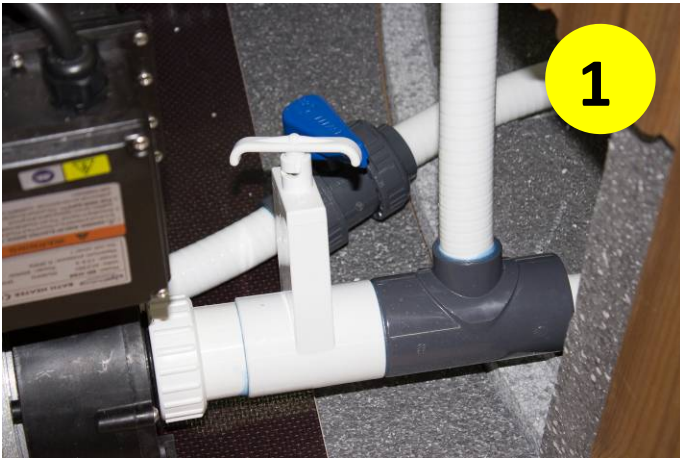
Press the handle down into the grooves
