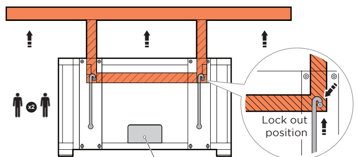
Fig.2 - Table in dining position.
