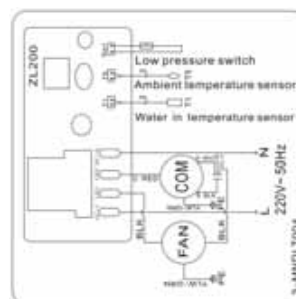
Heatermax COMPACT 10
