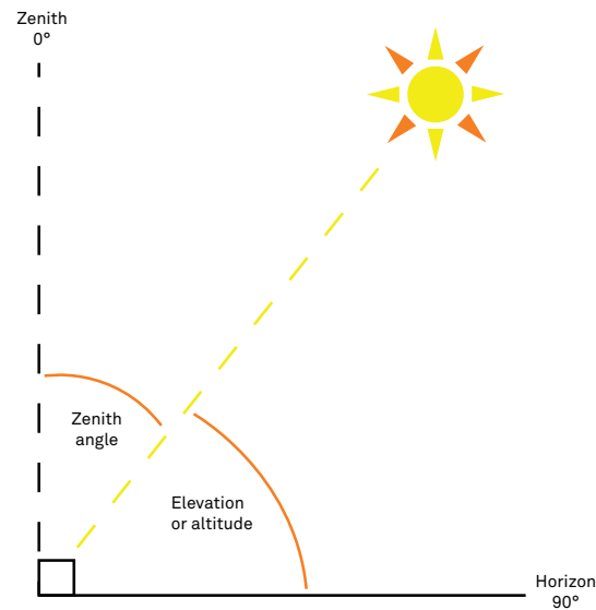
Figure 36 Zenith angle
