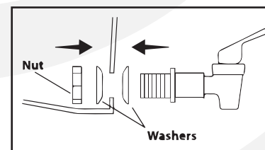
How to Install Spigot and Filter
