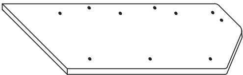
(2)/1PC Right Side Board SIZE: 43in. x 23in.
