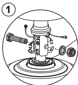
Secure Extension Tube & Tighten Hardware
