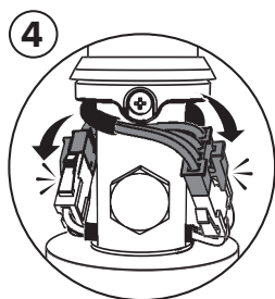
Plug In Wiring Harnesses
