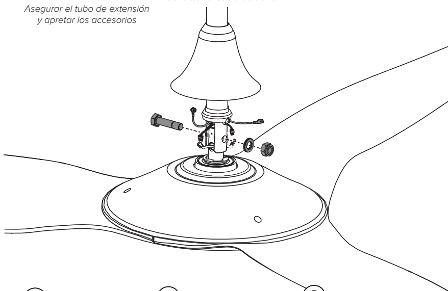
Secure Extension Tube & Tighten Hardware
