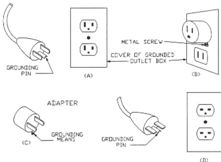
Fig. 1: Grounding Methods
