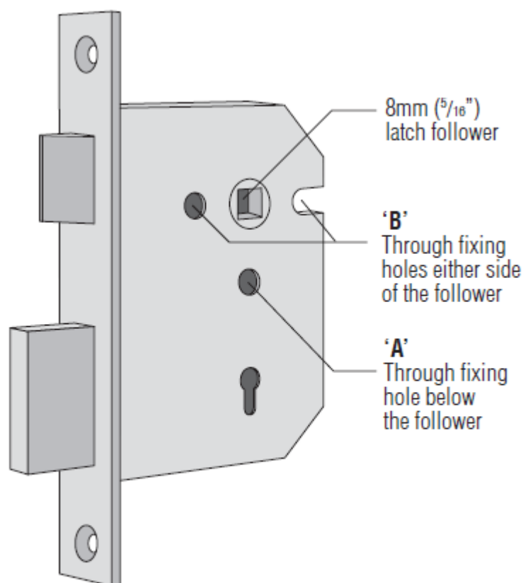
FIGURE 1 - Lock case
