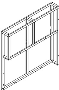
Right back frame (1 pc)
