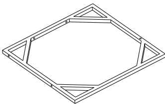
Seat frame H (2 pcs)
