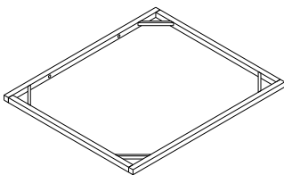
Seat frame (2 pcs)
