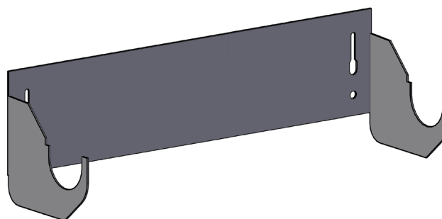
Figure 1-2: Lower mounting bracket for vertical Afinia radiators
