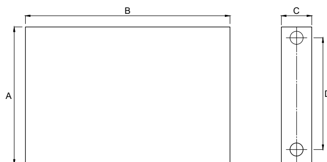
Figure 2-1: Radiator Dimensions
