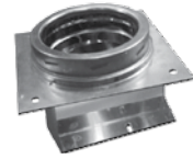
Anchor Box with DuraTech Anchor Plate (Model #6DT-AP, 6") * Works with Class A Stainless Steel DuraTech 6" Double Wall Pipe (model #6DT-24SS) to meet Standard HT 103
