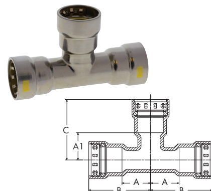
PCH211 Tee P x P x P – Carbon Steel
