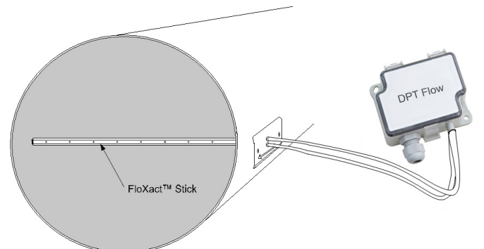
FloXact™-R mounting
