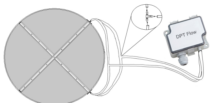
FloXact™-R mounting with two probes.
