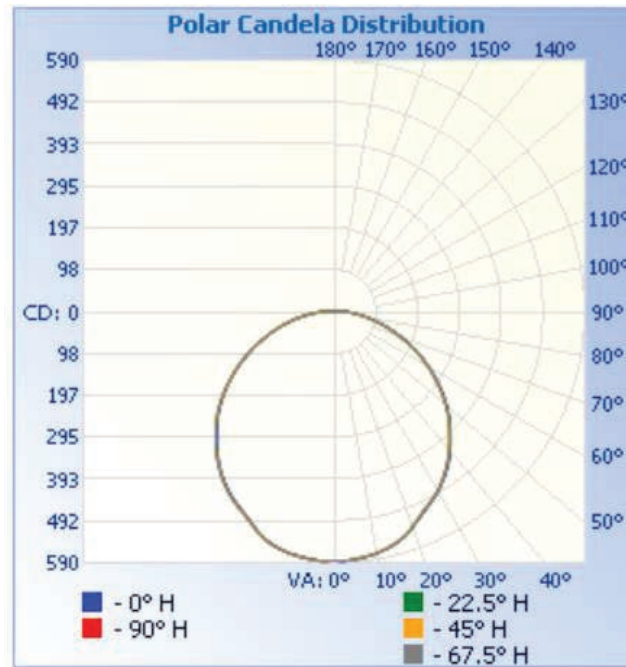
Light Distribution Curve
