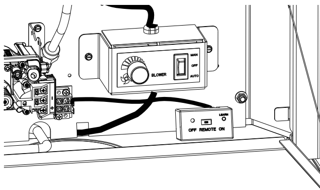
Figure 10.6. Remote Receiver Location. Shown with optional blower.
