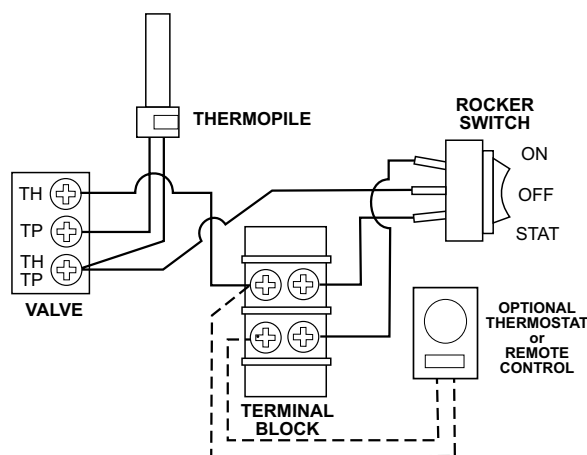
Figure 10.7. Accessory wiring diagram.
