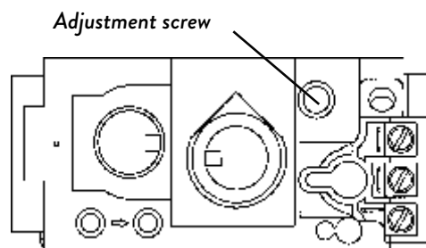
Figure 12.2. Pilot flame regulation.
