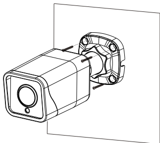
Figure 3-1 Installing camera
