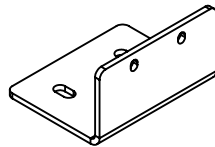
F45 MOUNTING BRACKET
