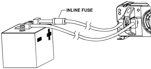
Figure 4. Battery Connections
