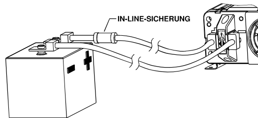
Abb. 4. Batterieanschlüsse
