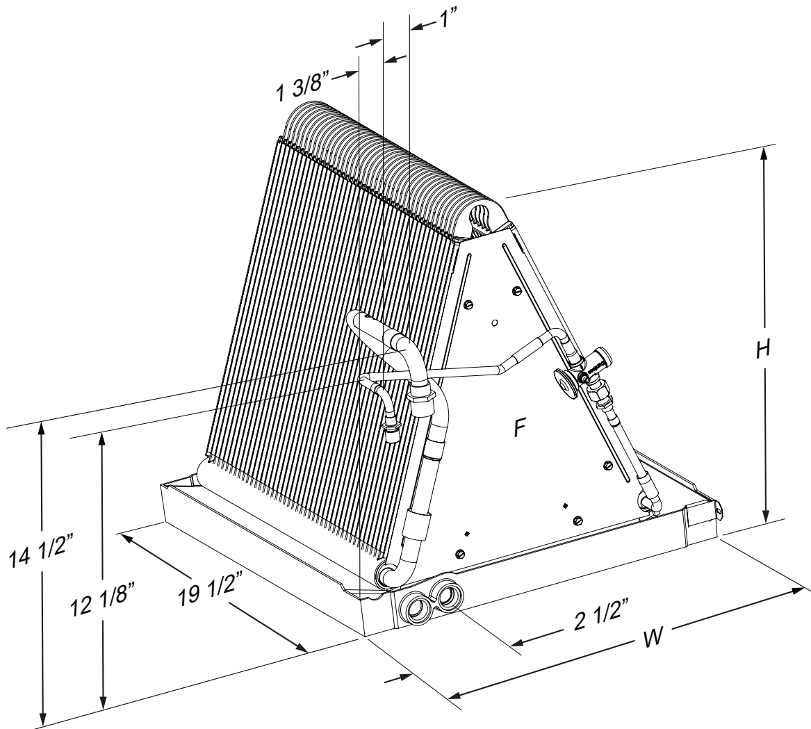
Figure 6. C84QA Coil Dimensions
