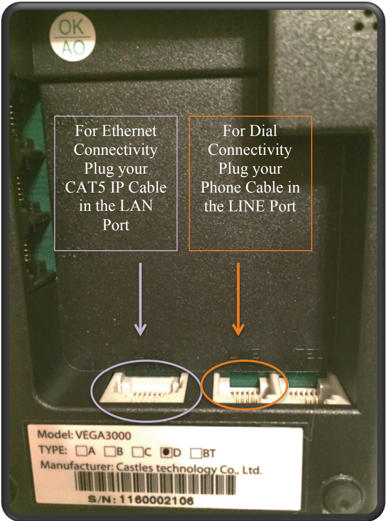
Underneath of Z9 Docking Station
