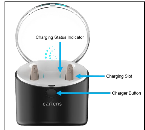
Figure 4: Earlens Charger
