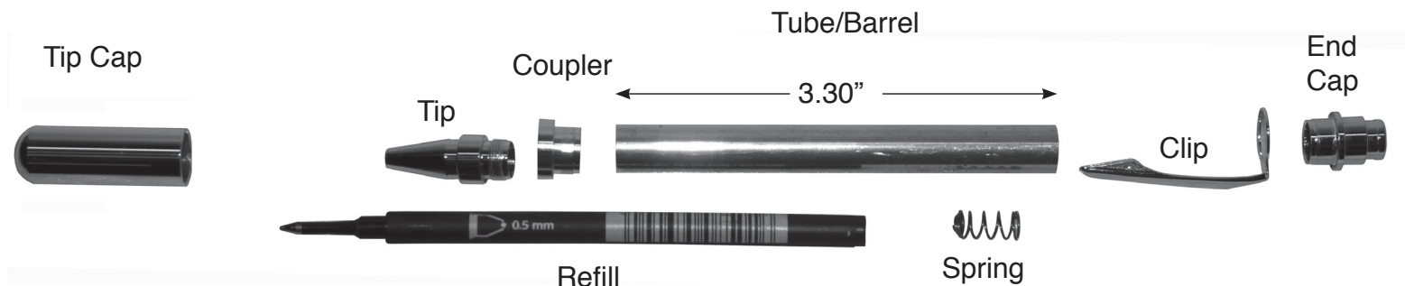
DIAGRAM A / PARTS LAYOUT
