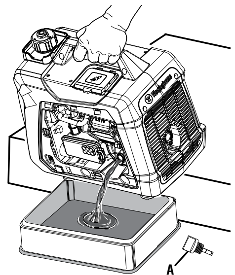
A - Oil dipstick
