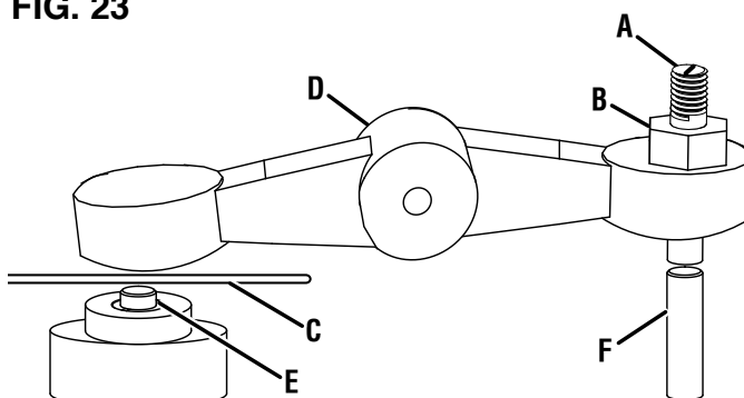
A - Adjustment Screw B - Jam Nut C - Feeler Gauge D - Rocker Arm E - Valve Stem F - Push Rod
