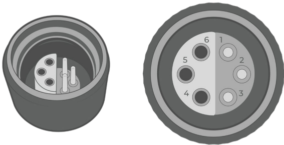
Figure 3: UW6 Receptacle pinout.
