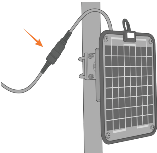
Figure 2: UW-6 Receptacle connection to a NexSens SP-Series Solar Power Pack.
