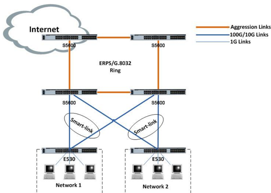
Figure 5-3 Metro L2 Ring Network topology with S5600 Series
