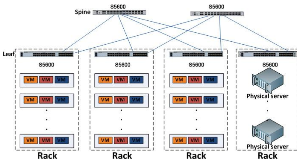
Figure 5-2 Data Center Servers Access Network with S5600 Series
