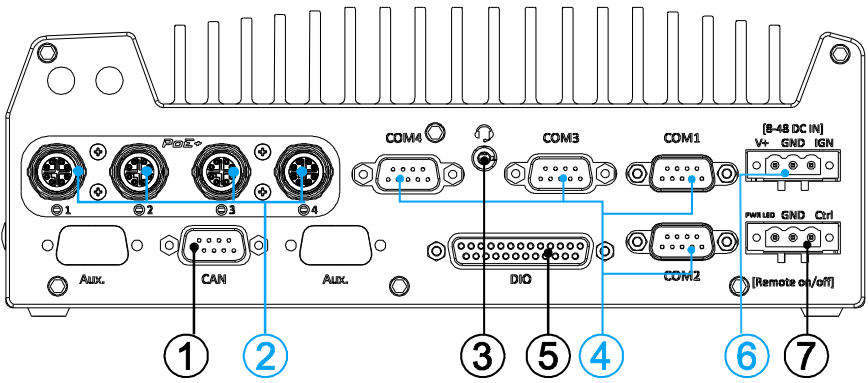
Nuvo-9100VTC
