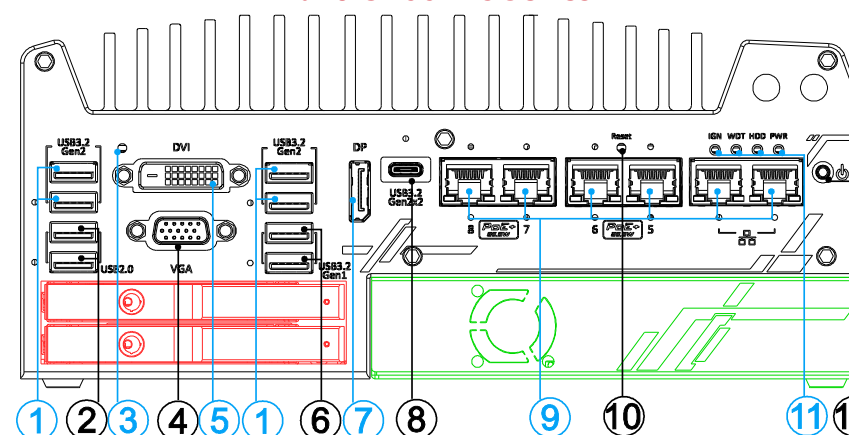
Nuvo-9100VTC Series
