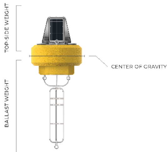
Figure 6: CB-450 buoyancy diagram.
