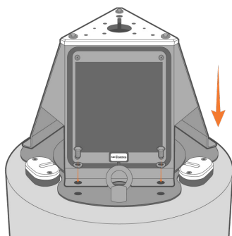
Figure 5: Solar tower installation.
