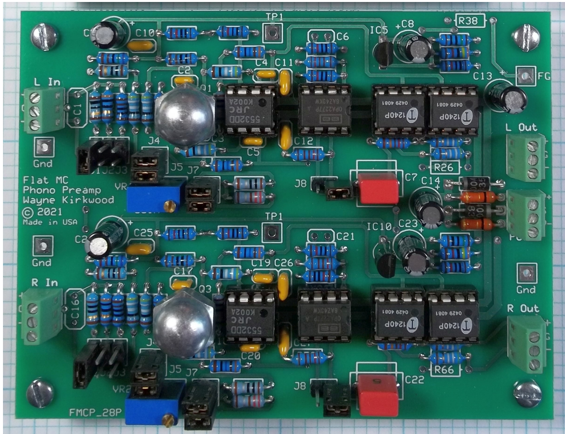
Flat MC Phono Preamp PC Board
