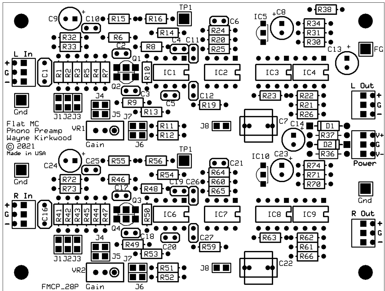
Flat moving coil preamp component and jumper placement.
