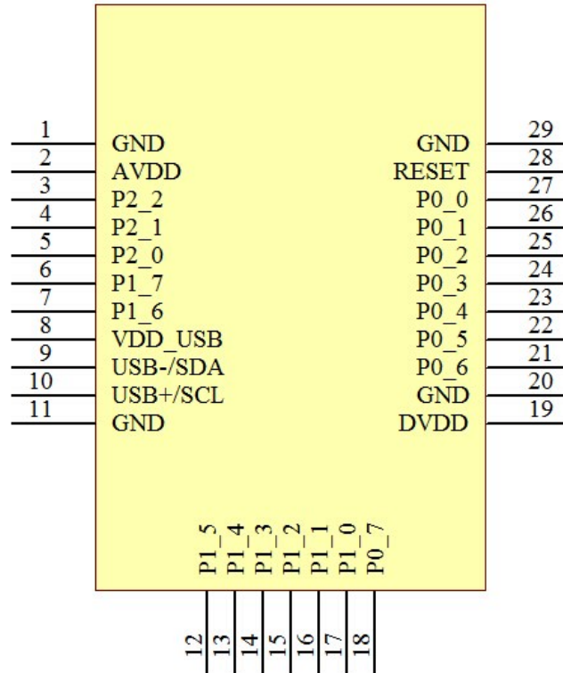
Fig. 3: The pinout of BDE-BLEM201 (TOP)
