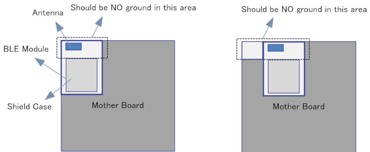
Fig. 4: Recommended location in X-Y plane
