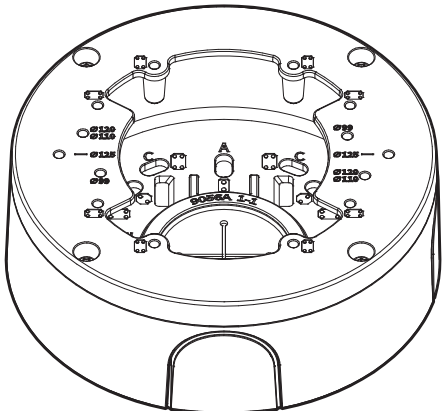
BACK BOX
