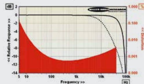
ABOVE: Distortion vs. freq. (red; balanced in/out re. 0dBV) and freq. resp. (dashed, with CD de-emphasis)
