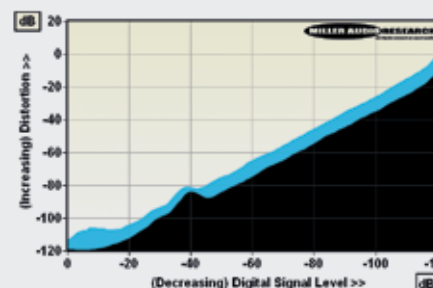
ABOVE: Distortion vs. 48kHz/24-bit digital signal level over a 120dB dynamic range (1kHz, black; 20kHz, blue)
